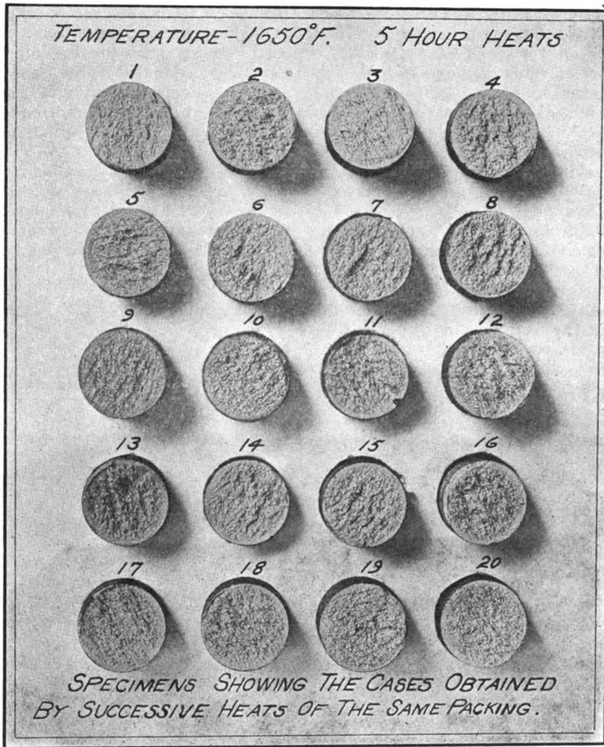
FIG. 5.—BROKEN SPECIMENS OF THE PIECES TREATED SHOWING THE CASE
