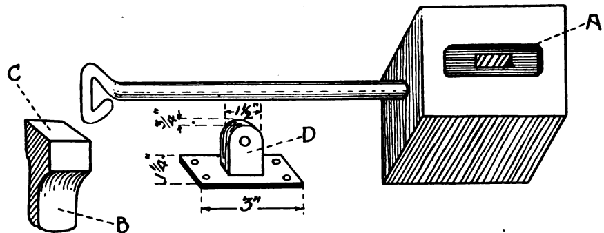
FIG. 3—TOOL FOR STAMPING PLATE WITH LUG
