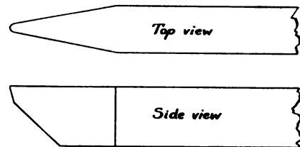
ROUND-NOSE TOOL FOR BRASS
