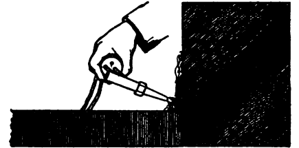
FIG. 1.—A DIFFICULT JOB AND HOW IT IS DONE. HOLDING THE TORCH IN THE RIGHT HAND HELPS TO DIRECT THE FLAME WITH GREATER ACCURACY IN TIGHT PLACES
