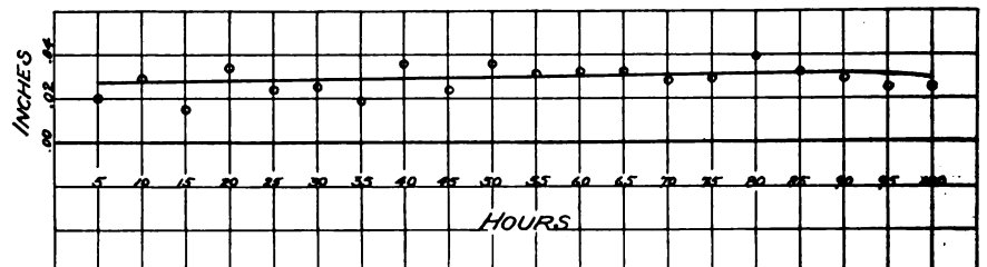
CURVE SHEET NO. 2 SHOWING RELATION BETWEEN THICKNESS OF CASE AND SUCCESSIVE HEATS OF PACKING
