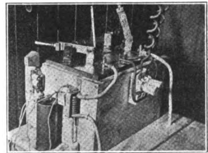
FIG. 7.—THE TRANSFORMER AND ITS FITTINGS
