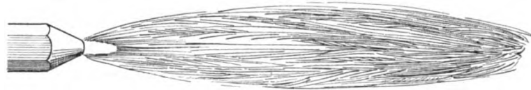
Properly adjusted or neutral welding flame. Cone in center is sharp and distinct, somewhat blunt. Ragged edges of the rosebud cone of the figure above just disappeared.
