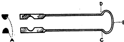
FIG. 9.—BOTTOM AND TOP FULLER
