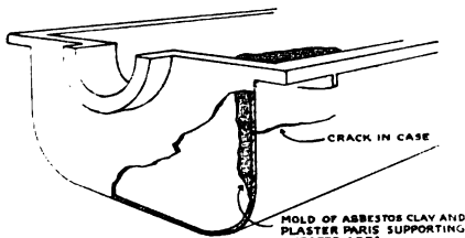
FIG. 4.—A BREAK CAN BE BACKED UP WITH A MOLD
