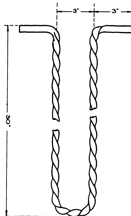
1—TWISTED BAR RE-INFORCEMENTS
