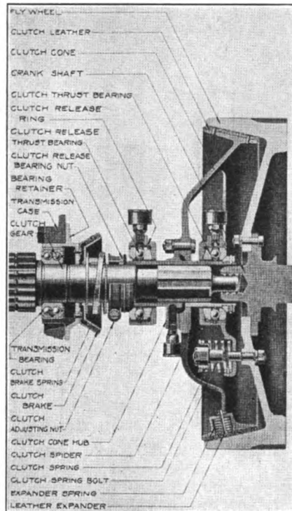
FIG. 1.—SECTIONAL VIEW OF BUICK CONE CLUTCH
