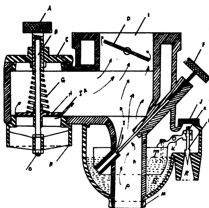
A SECTIONAL VIEW OF A TYPICAL AUTOMOBILE CARBURETOR
