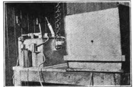
FIG. 10.—THE FURNACE HOOD, TRANSFORMER AT LEFT
