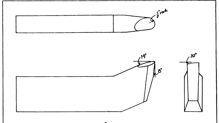
FIG. 1. THE TOOL TAKEN WAS A STANDARD CUTTING TOOL
