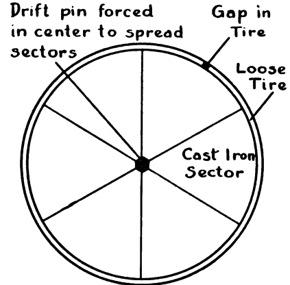
FIG. 5—FOR COLD BENDING SMALL JOBS
