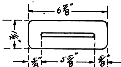
FIG. 1—DIMENSIONS FOR FLAT BAR USED IN FORGING WELDLESS RINGS
