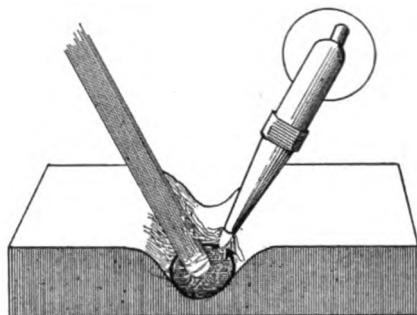
FIG. 2—IT IS NECESSARY TO KEEP THE TORCH IN MOTION, SWINGING AROUND IN TINY CIRCLES
