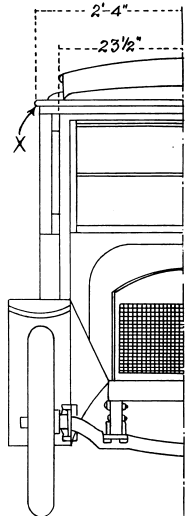
FIG. 3.—FRONT VIEW OF CAB SHOWING HOW LINES BLEND WITH BODY
