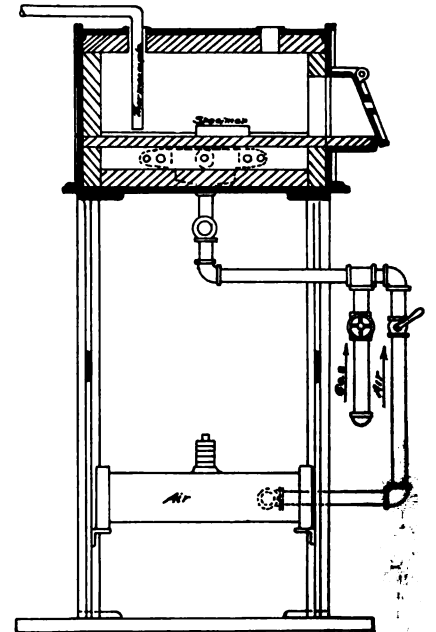
FIG. 2.—THE HEAT TREATMENT FURNACE SHOWING SECTIONAL VIEW OF HEATING OVEN
