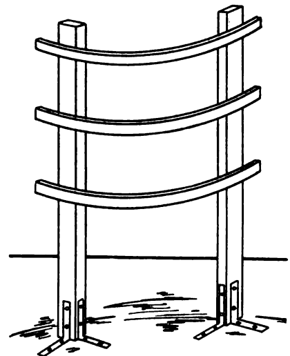
AN EASILY MADE MACHINE GUARD. STOCK: TWO UPRIGHTS 48"x2 3/4"x1 1/2" TWO BENT STRIPS 37"x1 1/2"x1 1/2"
