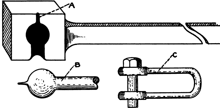
FIG. 2—BALLING-SWAGE
