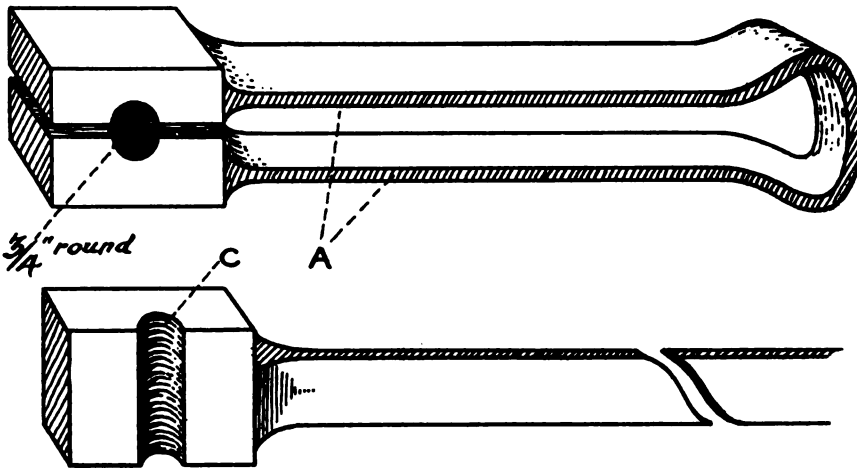
FIG. 1.—ROUND SWAGE
