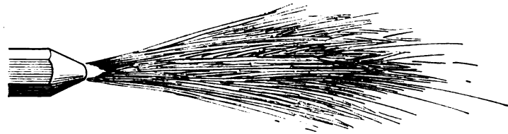
Too much oxygen in this flame, so it is termed an oxidizing one. Cone is shorter than in the above figure, more pointed and a different color, changing from the blue white to a darker blue. This flame is most easy to get and will ruin the weld.
