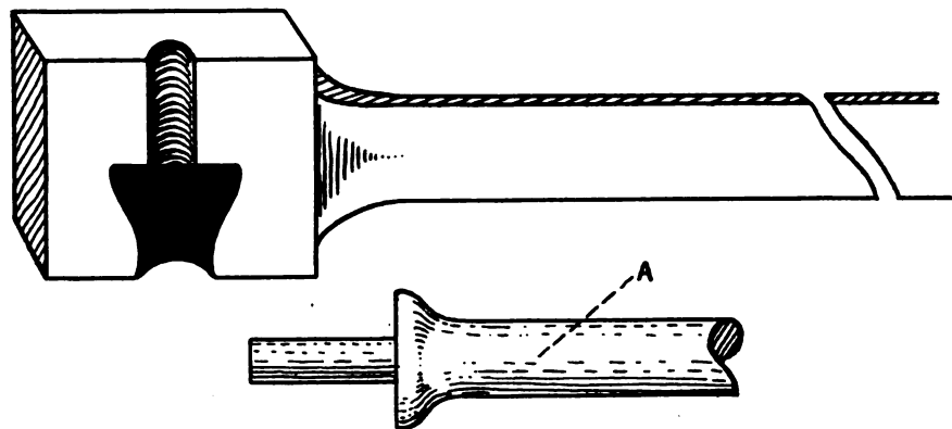
FIG. 3—COLLARING-SWAGE
