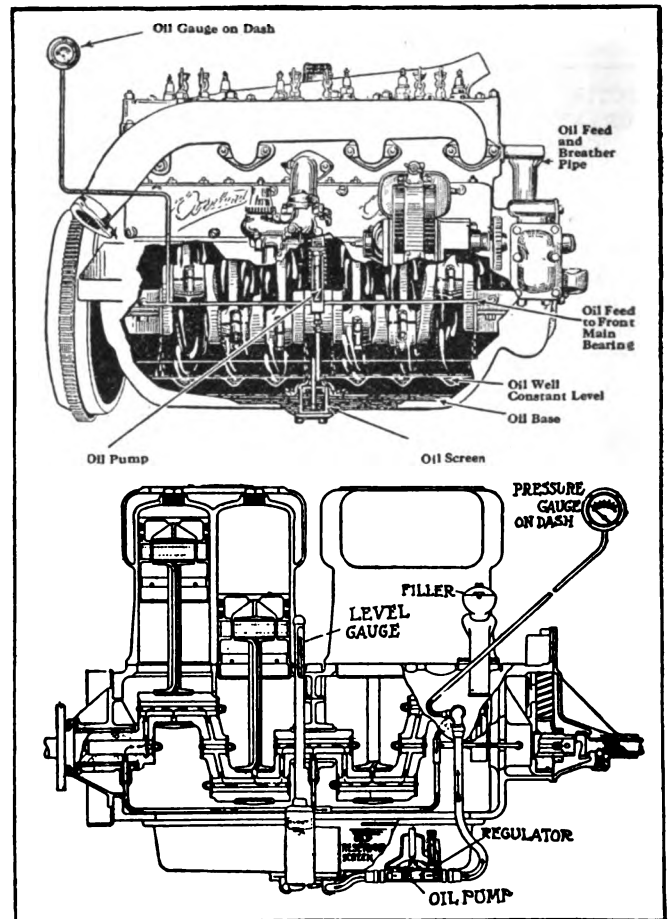
PART SECTIONAL VIEW AT TOP SHOWS OILING SYSTEM OF OVERLAND SIX MOTOR. BELOW THE PRESSURE FEED THROUGH OIL PASSAGES IN CRANKSHAFT OF MARMION FOUR CYLINDER
