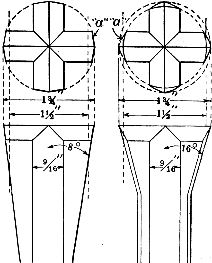
FIG. 2-A. TWO FORMS OF THE ORDINARY CROSS OR SQUARE BIT. THE CHIEF DISTINCTION IS IN THE TAPER, ONE BEING 8° AND THE OTHER 16°
