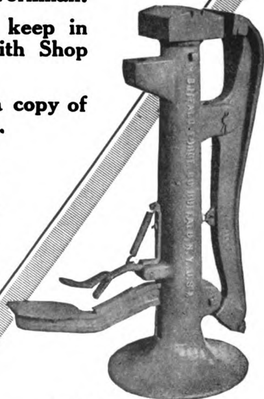
“SHOEMAKER” Vice. Saves time and labor on turning heels on shoes, hot filing, etc. Head 5 1/2" square—bevel on both sides. Leaves operator's hands free.
