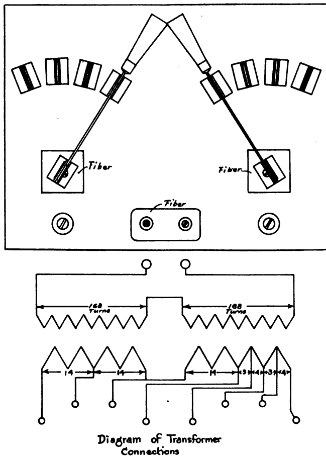
Diagram of Transformer Connections FIG. 5.—TOP VIEW OF THE SWITCH BOARD AND ALSO DIAGRAM OF CONNECTIONS
