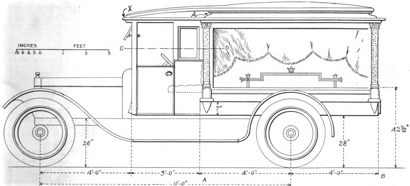
FIG. 1.—SIDE VIEW AND DIMENSIONS OF HORSE-DRAWN HEARSE BODY ADAPTED TO PIERCE-ARROW CHASSIS
