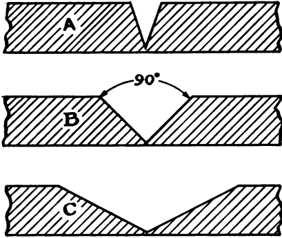
FIG. 2.—THE RIGHT AND THE WRONG WAY OF GROOVING: A—WRONG. A NARROW ANGLE IS HARD TO WORK AND MAKES A WEAK WELD. B—THE CORRECT ANGLE—ABOUT 90 DEGREES. C—WRONG. A WIDE ANGLE MAKES A WEAK JOINT AND REQUIRES TOO MUCH METAL.
