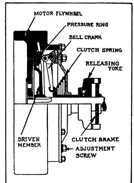
FIG. 2.—PART SECTIONAL VIEW OF BORG AND BECK THREE PLATE CLUTCH
