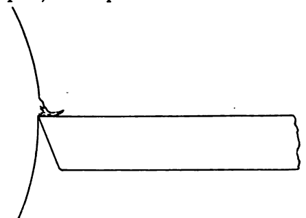
FIG. 3—FOR CUTTING BRASS THE TOP SURFACE OF THE TOOL IS LEVEL
