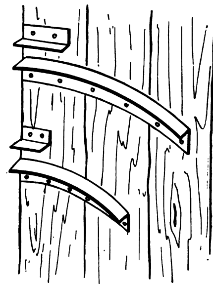
FIG. 8—TWO CURVES OF ANGLE-BARS. UPPER IS SHAPED ON A LONGER RADIUS THAN LOWER. THE TWO SMALLER PIECES ARE SHORT SECTIONS OF ANGLE-BARS. ALL FOUR ARE SECURED AGAINST A WOODEN WALL
