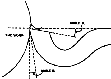
FIG. 4—A ROUGHING TOOL FOR HARD METAL
