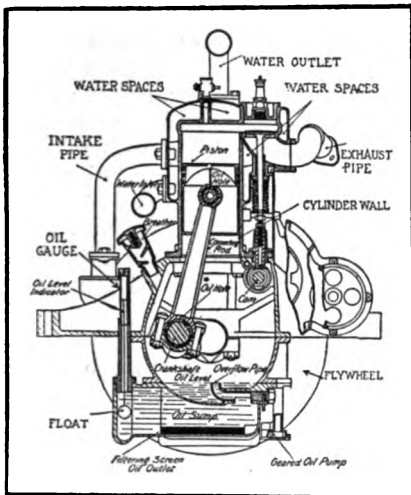
SECTION OF MOTOR CYLINDER AND CRANKCASE SHOWING PARTS OF CONSTANT LEVEL SPLASH LUBRICATING SYSTEM
