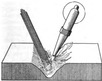
FIG. 1—KEEP THE ROD IN CONTACT WITH WELD AT ALL TIMES WHILE WORKING
