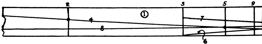
AN OLD PROBLEM: LAYING OUT A WOOD AXLE
