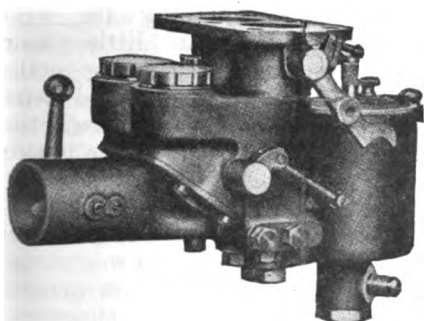
THE BALL & BALL CARBURETOR USED ON THE PEERLESS EIGHT IS OF THE DUPLEX MODEL, HAVING A SEPARATE VAPORIZING CHAMBER FOR EACH SET OF CYLINDERS
