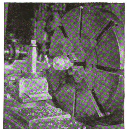
Fig. 118K. BUILDING UP OPERATIONS. (Note that the weld is easily machined). \frac{5}{32} '' Electrode, 130 Amp., 20 Volts will deposit one pound of metal in approximately 30 minutes. \frac{3}{16} '' Electrode, 175 Amp., 22 Volts will deposit one pound of metal in approximately 20 minutes. Using \frac{5}{32} '' Electrode, one cubic inch of steel may be deposited in about 7\frac{1}{2} minutes. The metal when deposited on mild steel by the metal electrode process will always be soft and easily machined. The carbon electrode process should be used for building up operations only when the built up piece can be later annealed to take out contraction strain.
