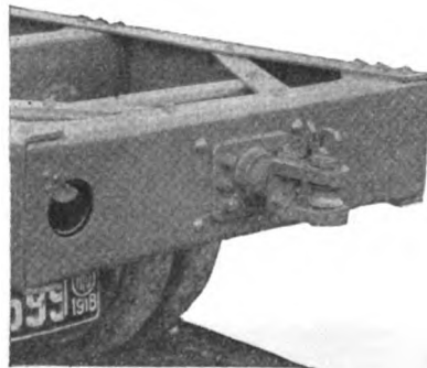
THE PROTECTED TAIL LIGHT AND SPRING DRAWBAR
