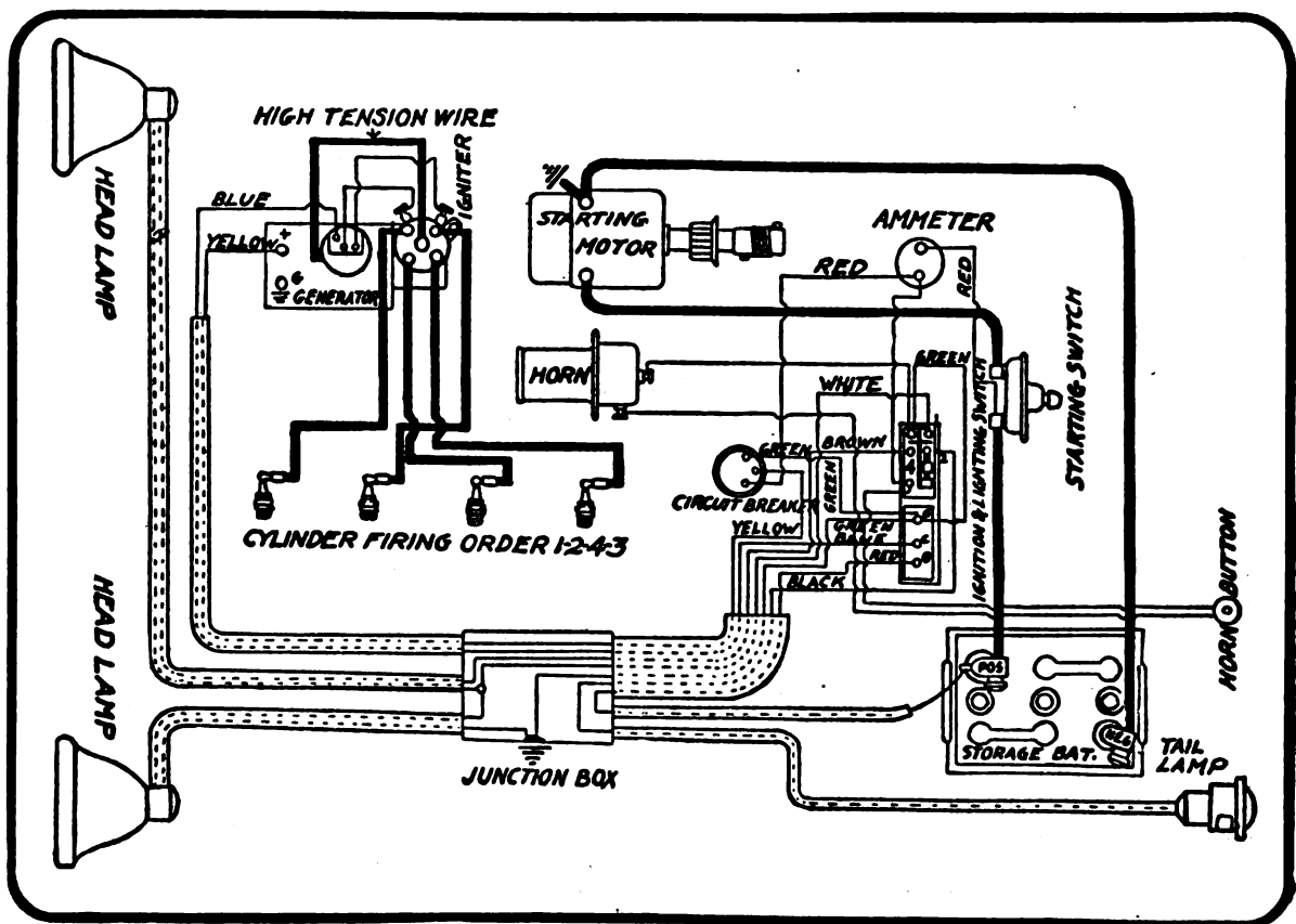
CHEVROLET "490" WIRING DIAGRAM
