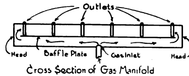
Cross Section of Gas Manifold
