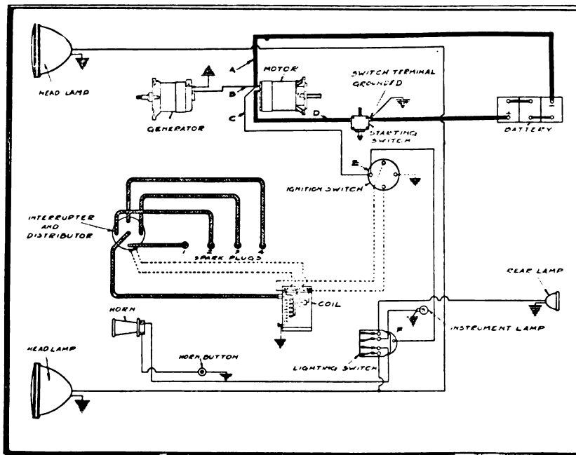
HUPMOBILE-BIJUR DIAGRAM
