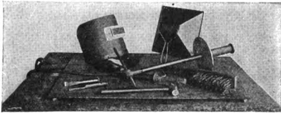
FIG. 142. OPERATOR'S TOOLS
