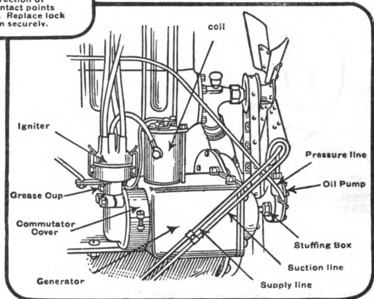
GENERATOR AND IGNITION SET
