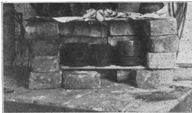
THE HEATING OVEN FOR "GROWING" PISTONS. THERE ARE CASES ON RECORD WHERE PISTONS HAVE BEEN INCREASED 1/64 WHICH IS USUALLY SUFFICIENT TO MEET ALL REQUIREMENTS FOR OVERSIZE PISTONS
