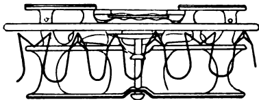
FIG. 2—RAKER GAUGE CUTTING DOWN RAKERS
