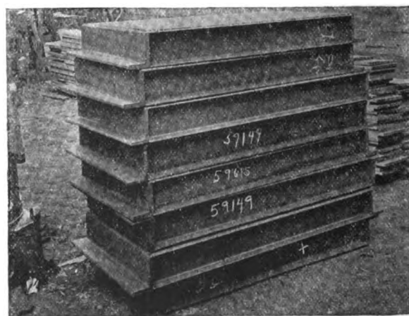
Fig. 115—Steel Machinery Bed-plates manufactured by use of the Arc Welder
