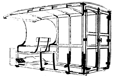
FULL PANEL BODY, CURVED SIDES AND ENDS
