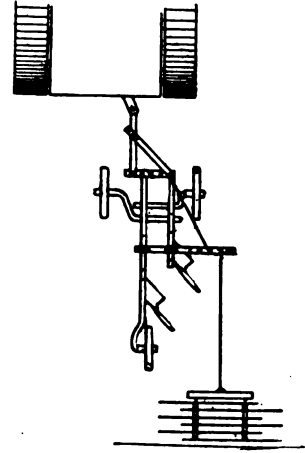
HITCH FOR TWO PLOWS AND HARROW
