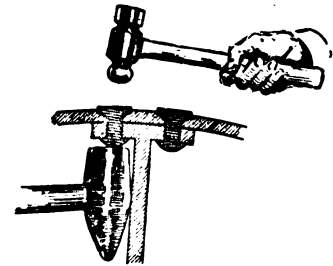
KEEP THE SPOKE RIVETS TIGHT
