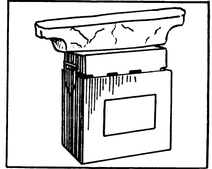
40—Place the wooden form over the covers and place a heavy weight on top of the form. The battery should stand for ten or fifteen minutes until the sealing compound has cooled and set. This can be scraped off with hot putty knife.
