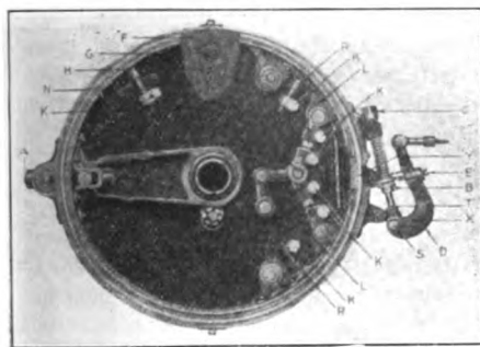
Interior View of Cadillac Brake Drum.
