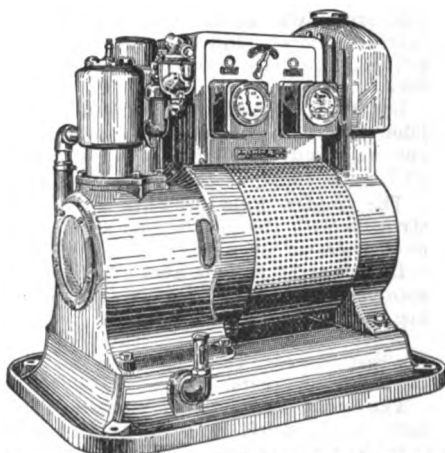
OWEN LIGHTING AND POWER UNIT FOR FARMS AND COUNTRY PLACCS
