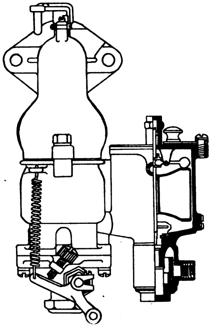
STEWART CARBURETOR
