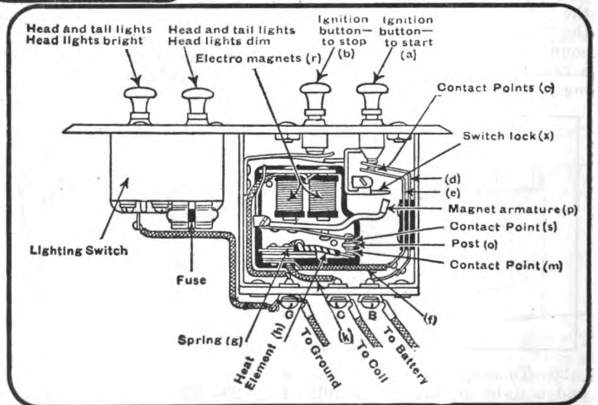
IGNITION SWITCH AND AUTOMATIC CUT-OUT
