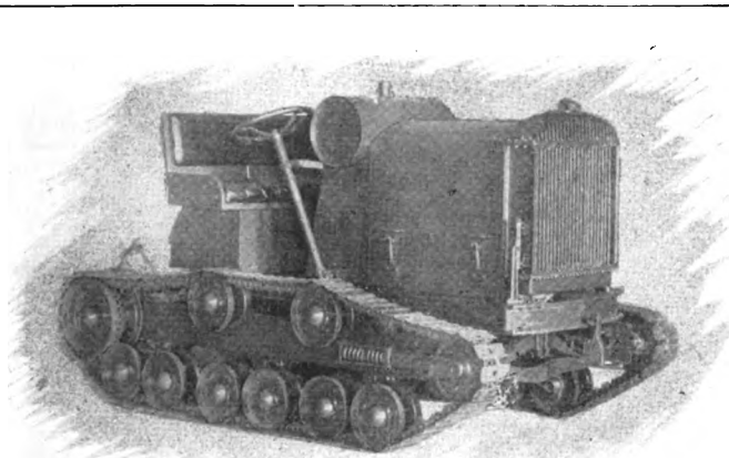
C. H. MARTIN IS THE INVENTOR OF THIS SIMPLE APPEARING TRACK LAYING TYPE TRACTOR DESIGNED TO PULL THREE PLOWS. OBSERVE THE ABSENCE OF THE MANY TRAPPINGS USUALLY FOUND AND THE AMPLE COMFORT SUGGESTED BY THE WIDE, UPHOLSTERED SEAT. THE TREAD IS MADE ENTIRELY OF PRESSED STEEL WHICH MEANS LIGHT WEIGHT AND GREAT STRENGTH AS WELL AS ECONOMY IN CONSTRUCTION COSTS
