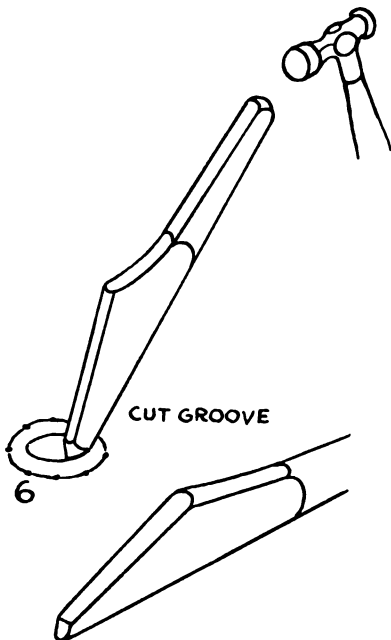
CHISEL AND METHOD OF TRUING UP AN OFF CENTER HOLE
