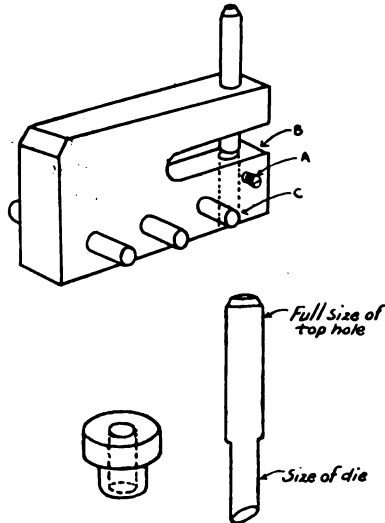
PUNCH DETAILS
