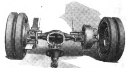
DOUBLE REDUCTION AXLE DISASSEMBLED
