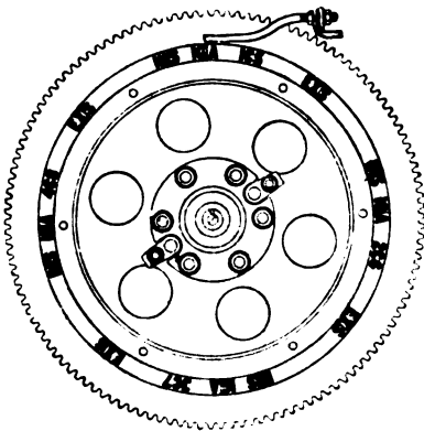
FLYWHEEL MARKINGS ON CADILLAC AUTOMOBILES
