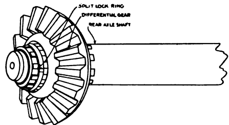
REMOVING DIFFERENTIAL GEAR
