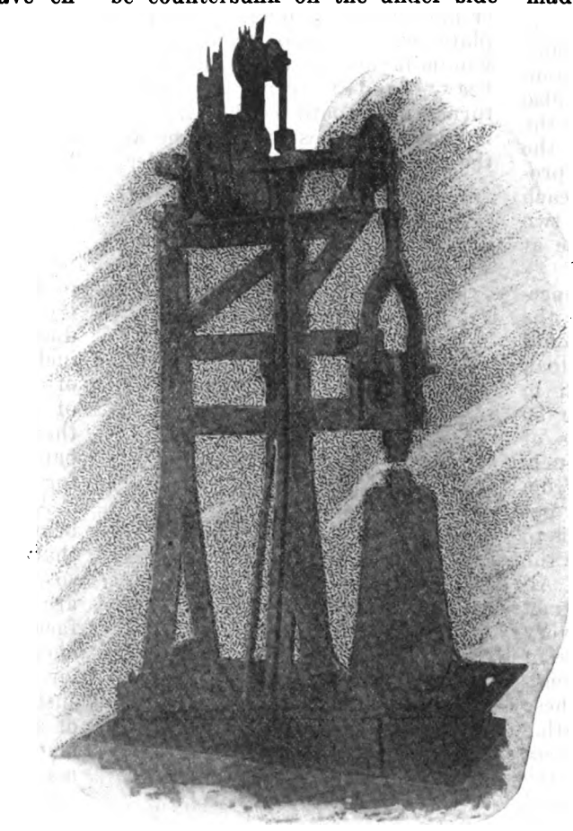
MR. WAGNER'S POWER HAMMER COMPLETED AND READY FOR WORK
