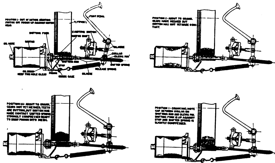
OPERATION OF HUPMOBILE STARTER
