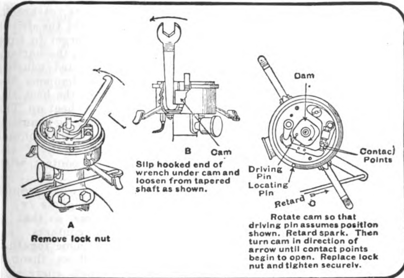
TIMING IGNITER
