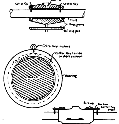
KEEPING OIL FROM SHAFTING
