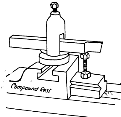
TOOL POST JACK
