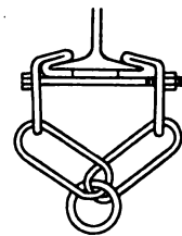
HOISTING TACKLE
