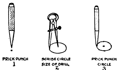
PROGRESSIVE STEPS IN LAYING OUT THE HOLE
