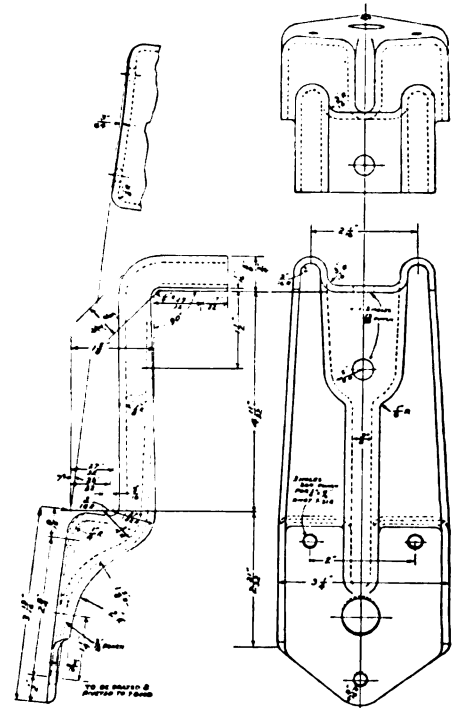
FORD CRANK CASE SUPPORT—FRONT
