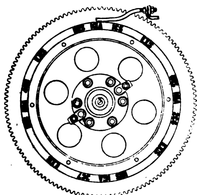
FLYWHEEL MARKINGS ON CADILLAC AUTOMOBILES
