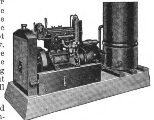
THE MATTHEWS IS ANOTHER AUTOMATIC SYSTEM AND NATURALLY REQUIRES A MINIMUM OF ATTENTION
